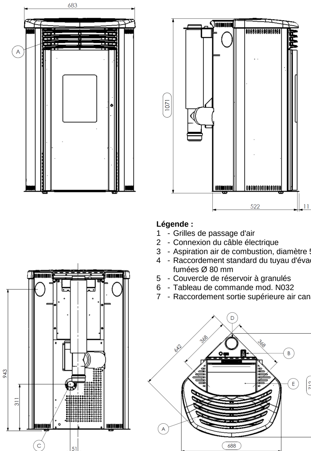
MIMOSA CAN. pellet stove dimensions
