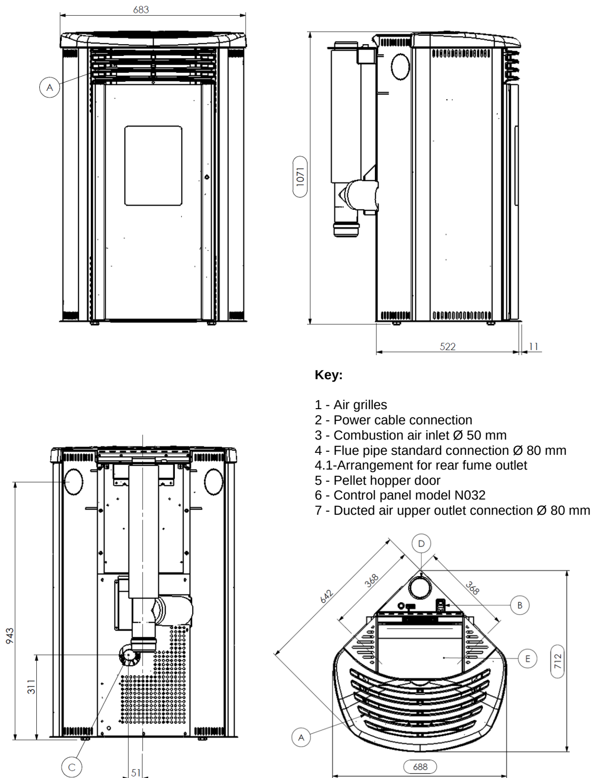
MIMOSA CAN. pellet stove dimensions
