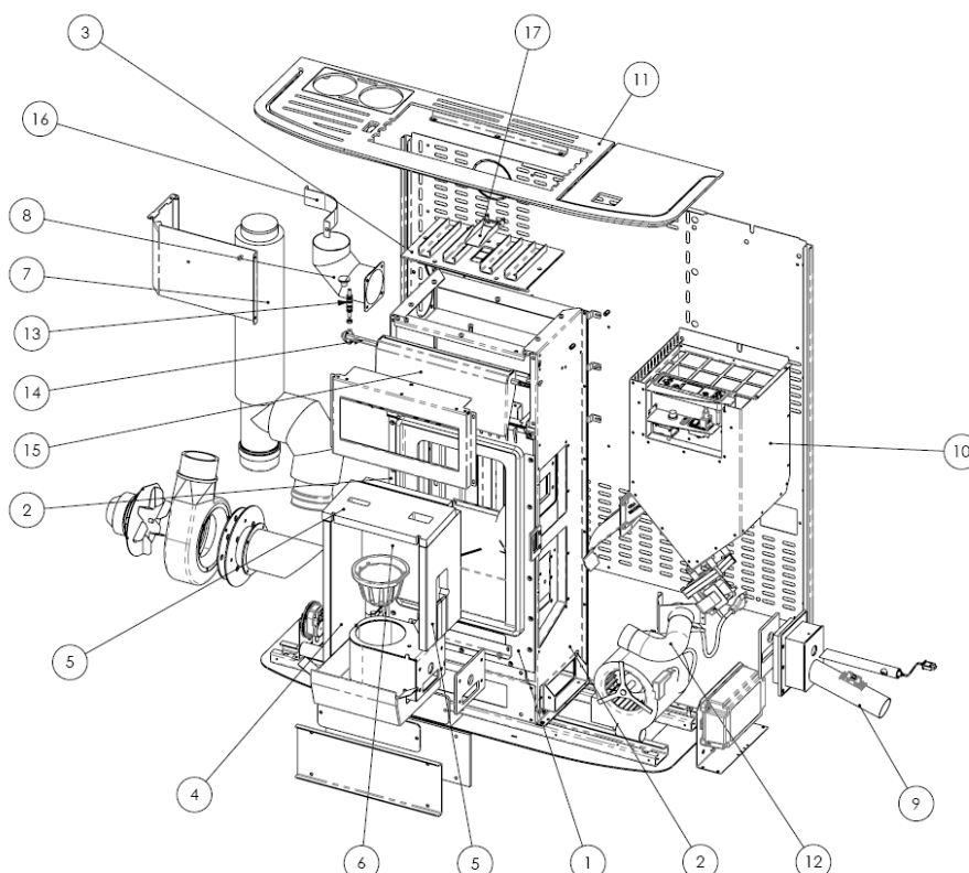
Exploded view of SPRINT** stove combustion chamber and parts
