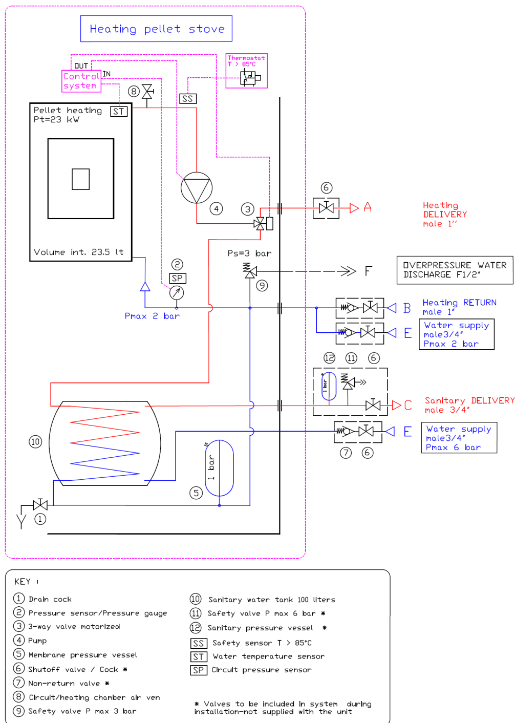
Hydraulic diagram - heating pellet stove 23 kW_04-2015
